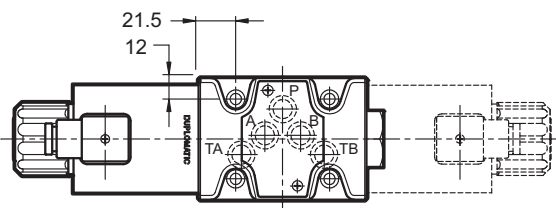
A*SB and C*SB versions solenoid position
