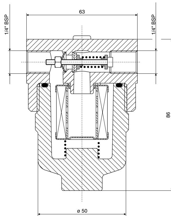
FILTRO COMPLETO CON BY-PASS COMPLETE FILTER WITH BY-PASS
