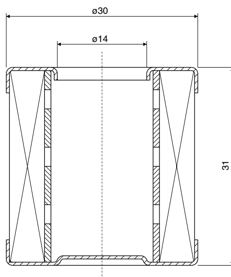
ELEMENTO FILTRANTE / FILTER ELEMENT
