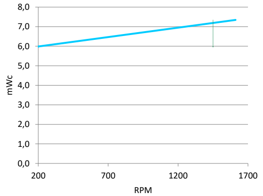
A) - NPSH required
