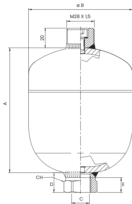
Technical drawing / Fluid connection G - M - Y
