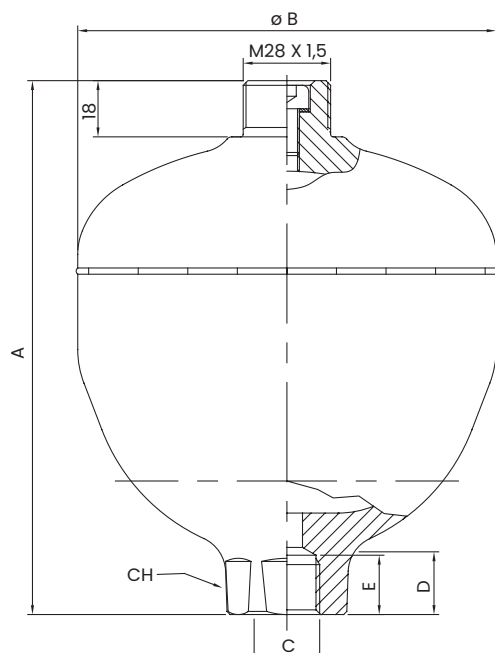
Technical drawing / Fluid connection G
